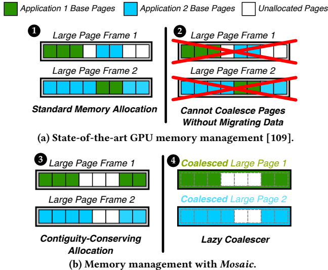
Figure 1: Page allocation and coalescing behavior of GPU memory managers: (a) state-of-the-art [109], (b) Mosaic.
