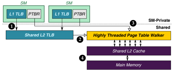
Figure 2: GPU-MMU baseline design with a two-level TLB.
