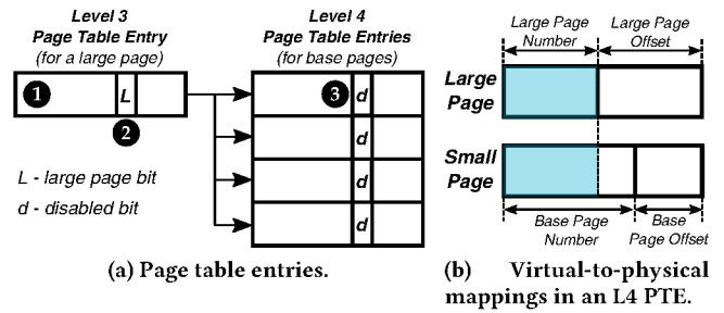
Figure 7: L3 and L4 page table structure in Mosaic .
