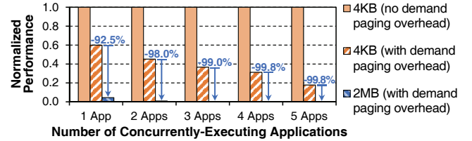
Figure 4: Performance impact of system I/O bus transfer during demand paging for base pages and large pages, normalized to base page performance with no demand paging overhead.
