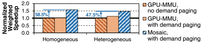
Figure 12: Performance of GPU-MMU and Mosaic compared to GPU-MMU without demand paging.
