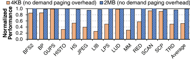
Figure 3: Performance of a GPU with no demand paging overhead, using (1) 4KB base pages and (2) 2MB large pages, normalized to the performance of a GPU with an ideal TLB.
